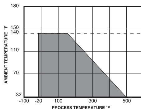
Figure 1. Ambient Temperature Range for Locally Mounted Electronics.
